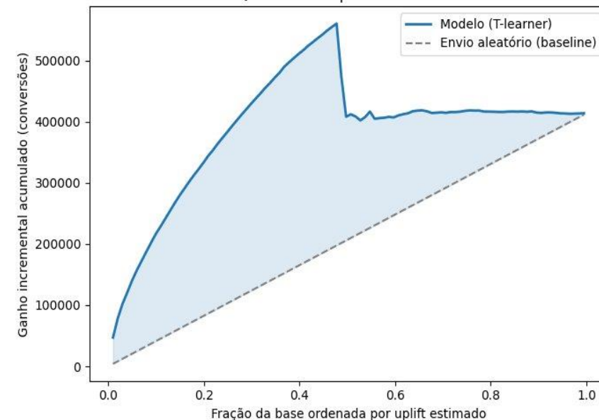
Qini Curve - Uplift do T-learner
